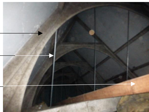
View in roof space showing trusses, ceiling beams and metal ties
