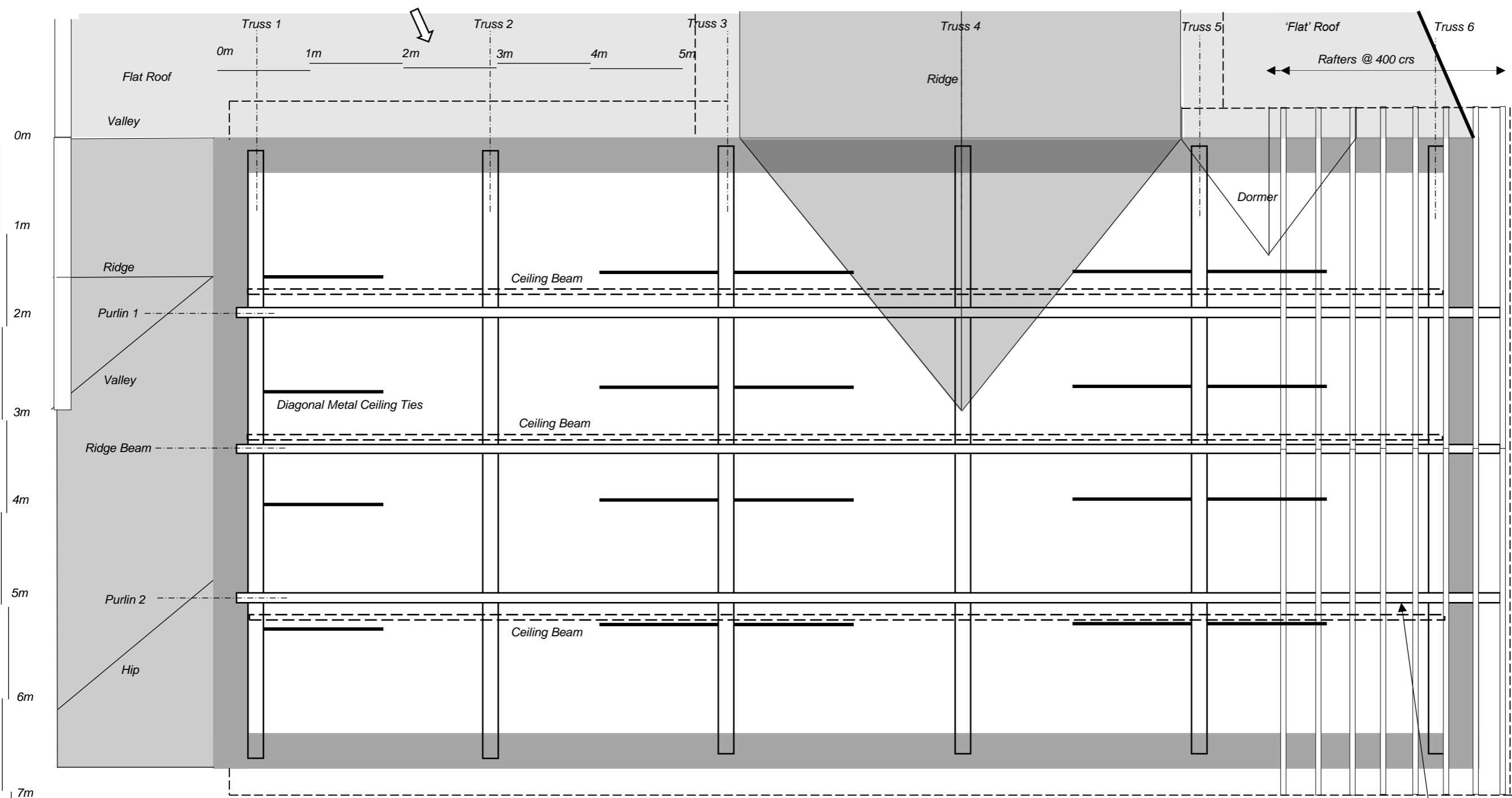
Roof edge/perimeter
